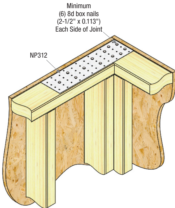
Typical NP312 prescriptive top-plate wall corner connection
