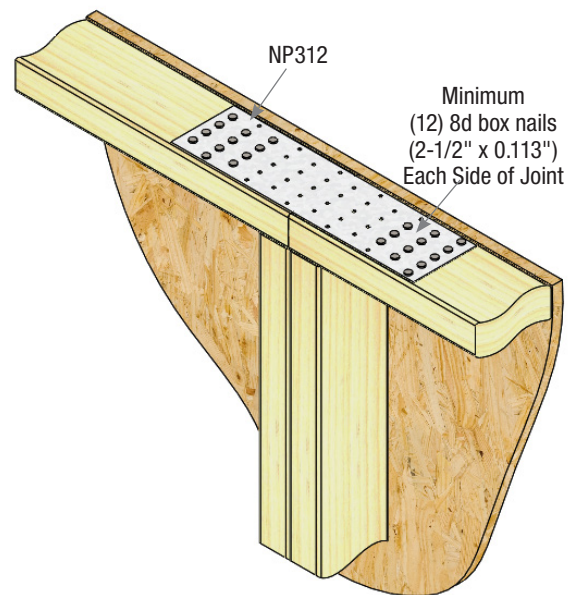
Typical NP312 prescriptive top-plate butt joint straight wall connection
