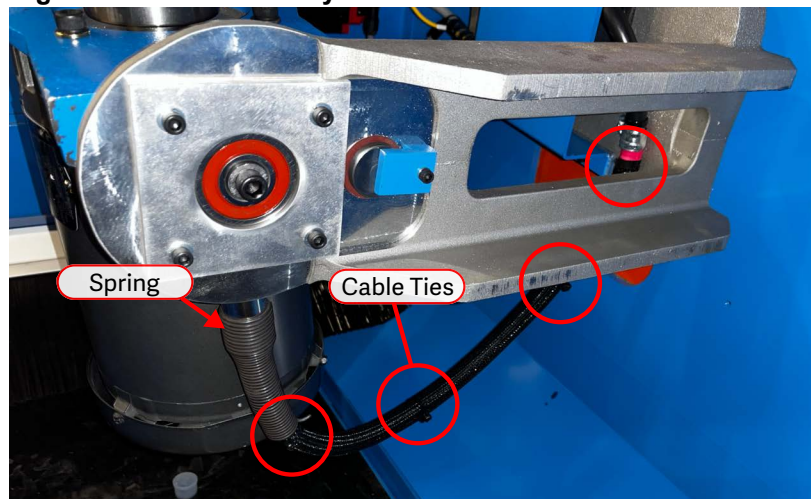
Figure 6: Cable Assembly
