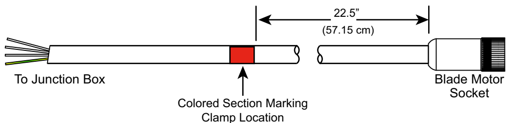
Figure 4: Blade Motor Cable Overview
