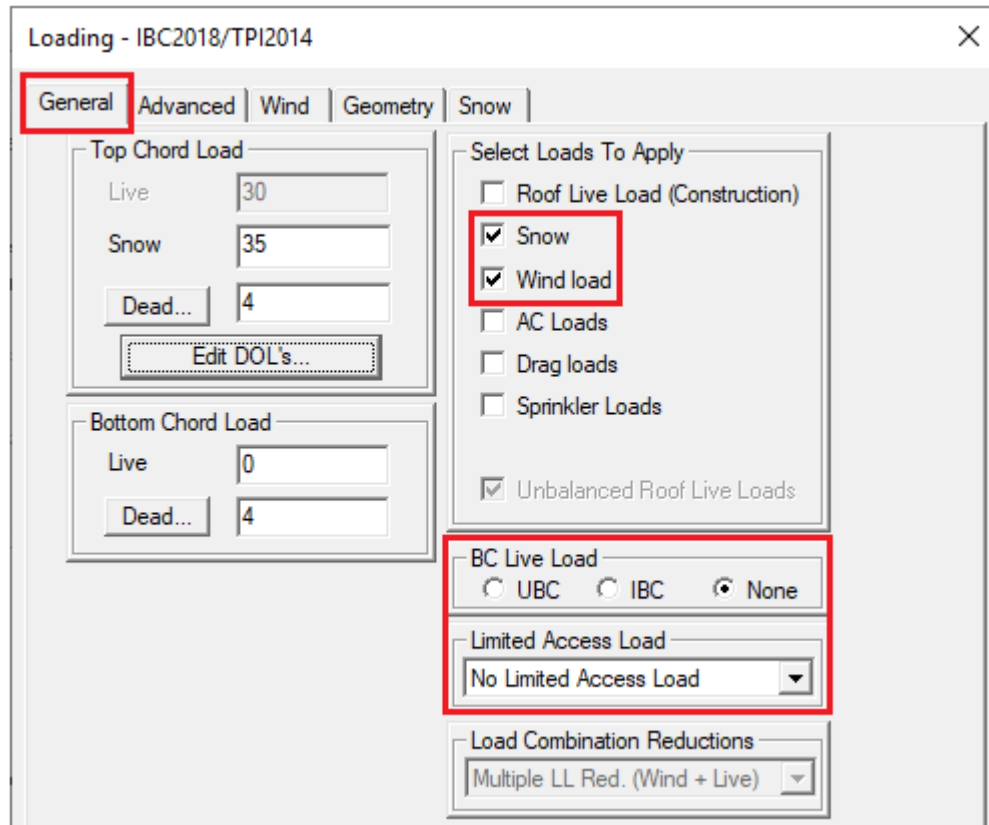
Figure 2 - General Loading Tab
