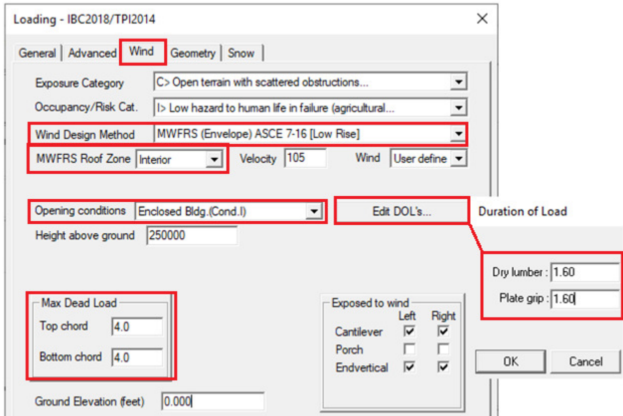
Figure 6 - Wind Loading Tab
