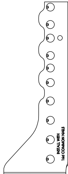
THDH612 - SIDE VIEW
