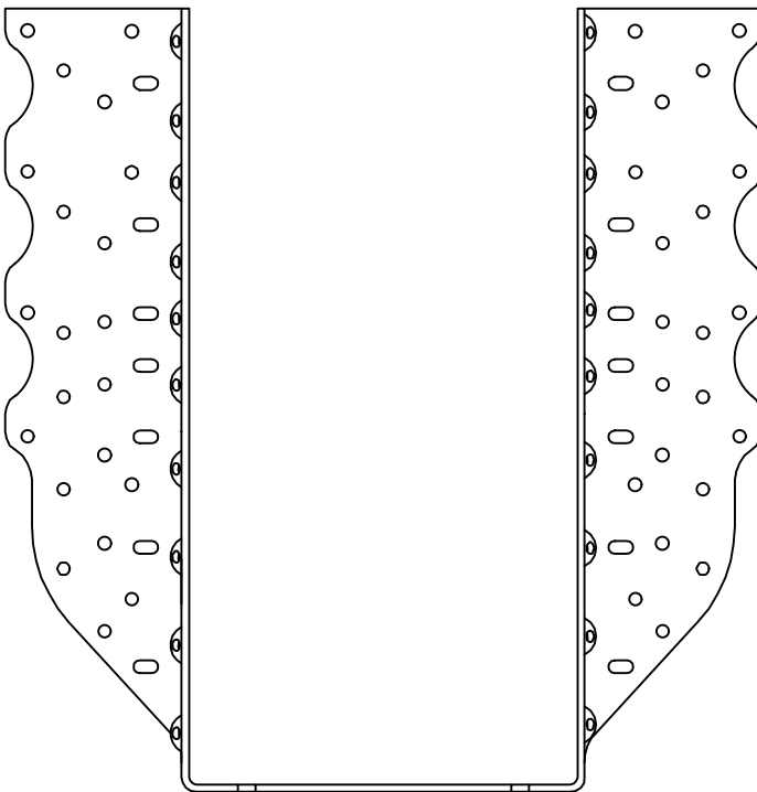
THDH612 - FRONT VIEW
