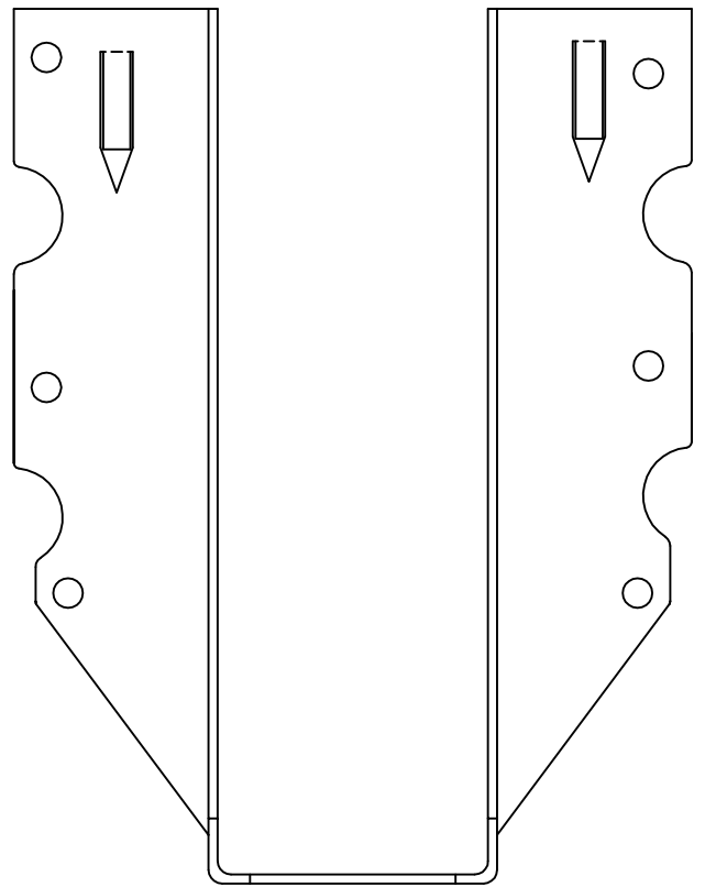
SUH26 - FRONT VIEW
