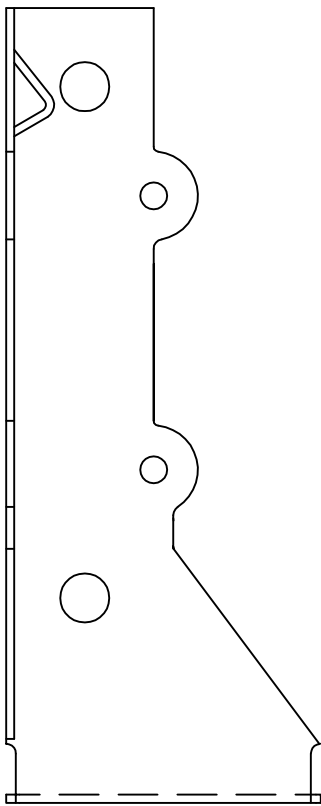
SUH26 - SIDE VIEW
