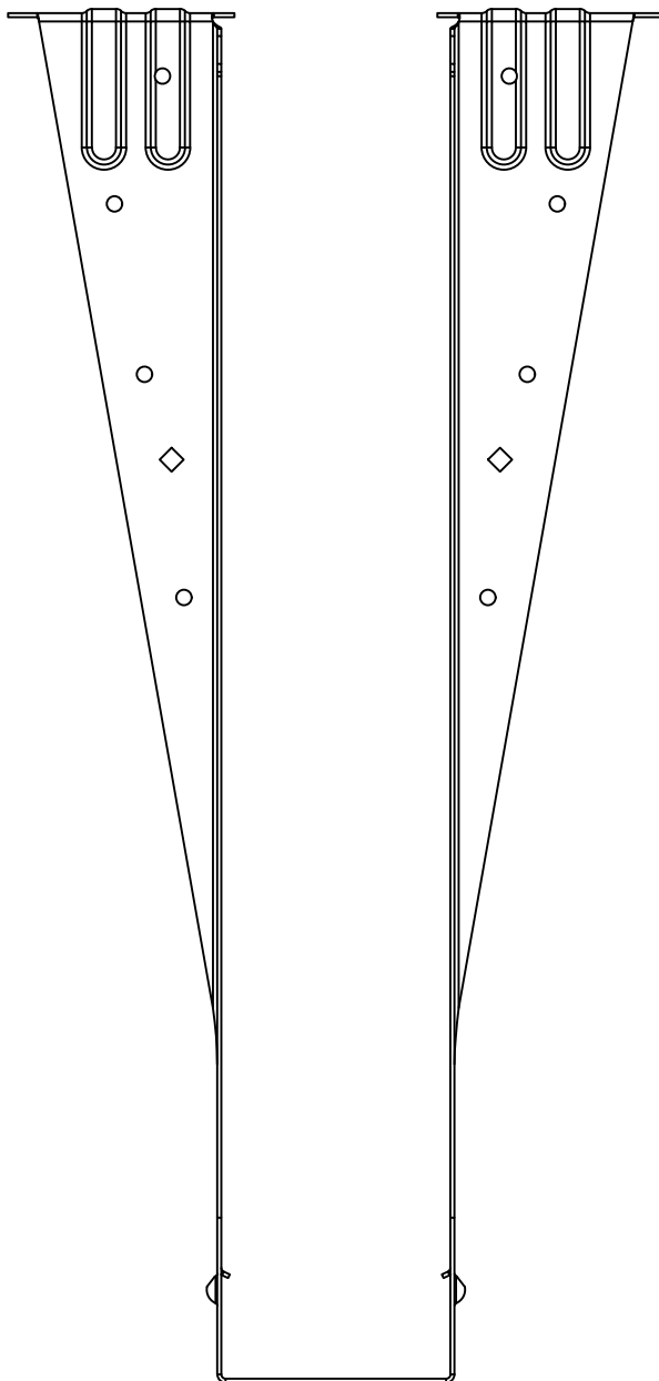
THO26160 - FRONT VIEW
