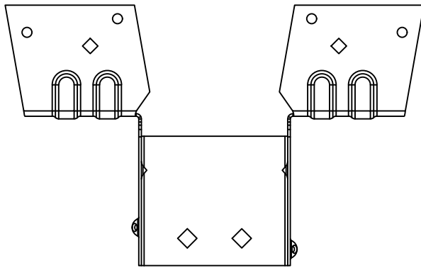
THO26160 - TOP VIEW
