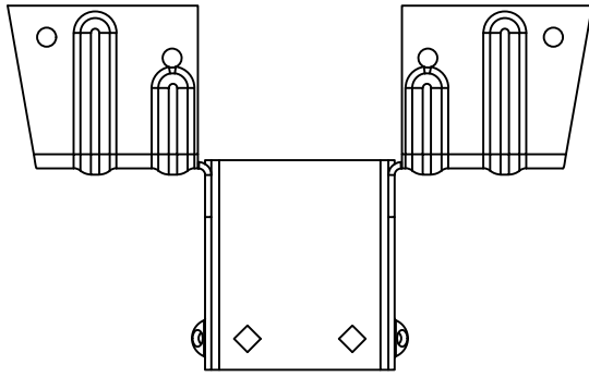
TH016112 - TOP VIEW
