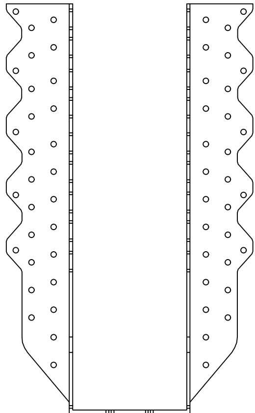
THD414 - FRONT VIEW
