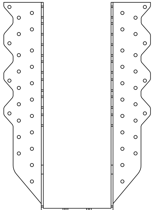
THD412 - FRONT VIEW
