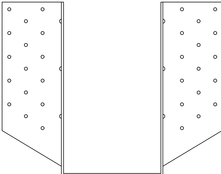
THD210-3 - FRONT VIEW
