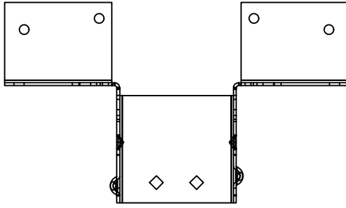
TFL2014 - TOP VIEW
