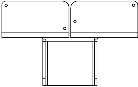
PHXU35925 - TOP VIEW
