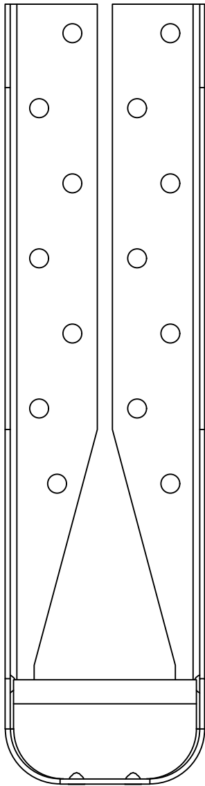
PHD5A - FRONT VIEW
