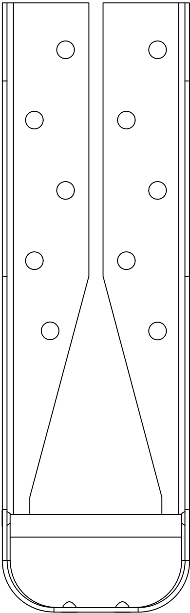
PHD4A - FRONT VIEW
