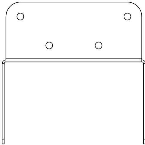
PB44-6TZ - FRONT VIEW
