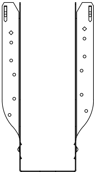
IHFL35112 - FRONT VIEW
