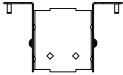
IHFL2314 - TOP VIEW
