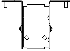
IHFL15112 - TOP VIEW
