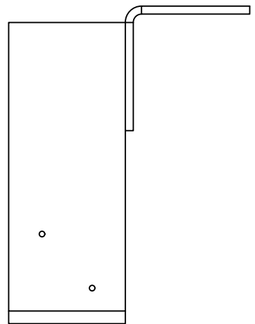
HWUH810 - SIDE VIEW
