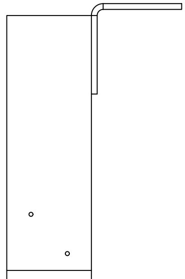
HWUH612 - SIDE VIEW
