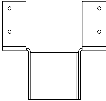
HDO314 - TOP VIEW
