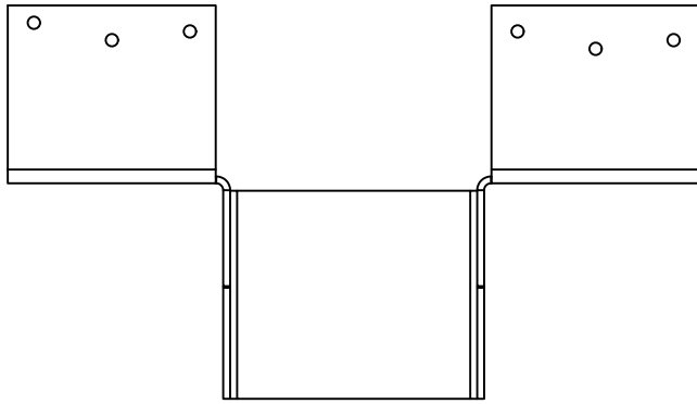
BPHA3514 - TOP VIEW
