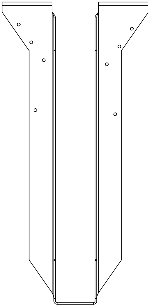
BPHA2318 - FRONT VIEW
