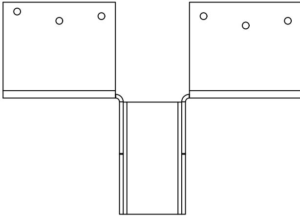
BPHA1514 - TOP VIEW
