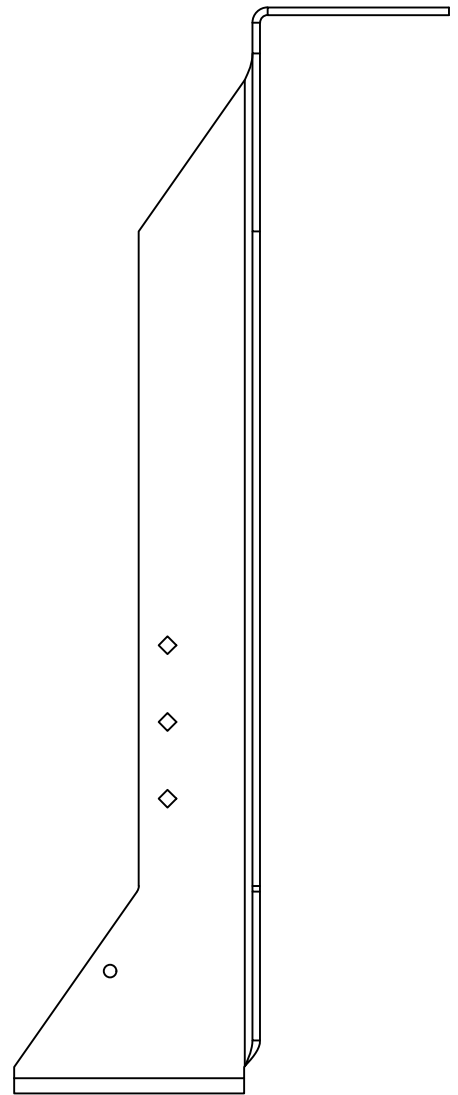
BPHA1514 - SIDE VIEW
