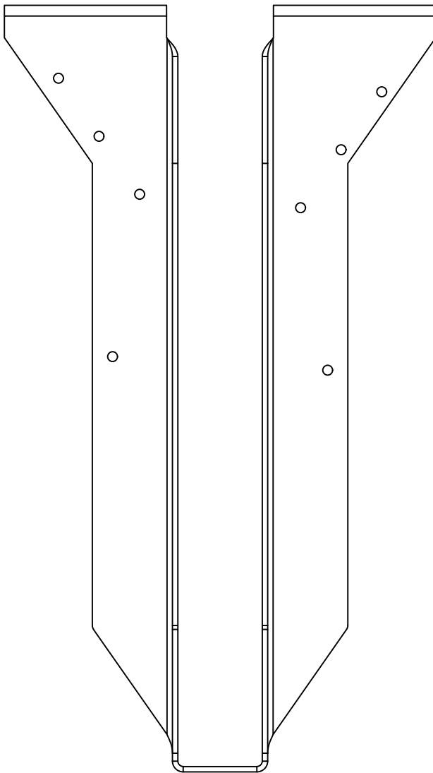
BPHA1514 - FRONT VIEW
