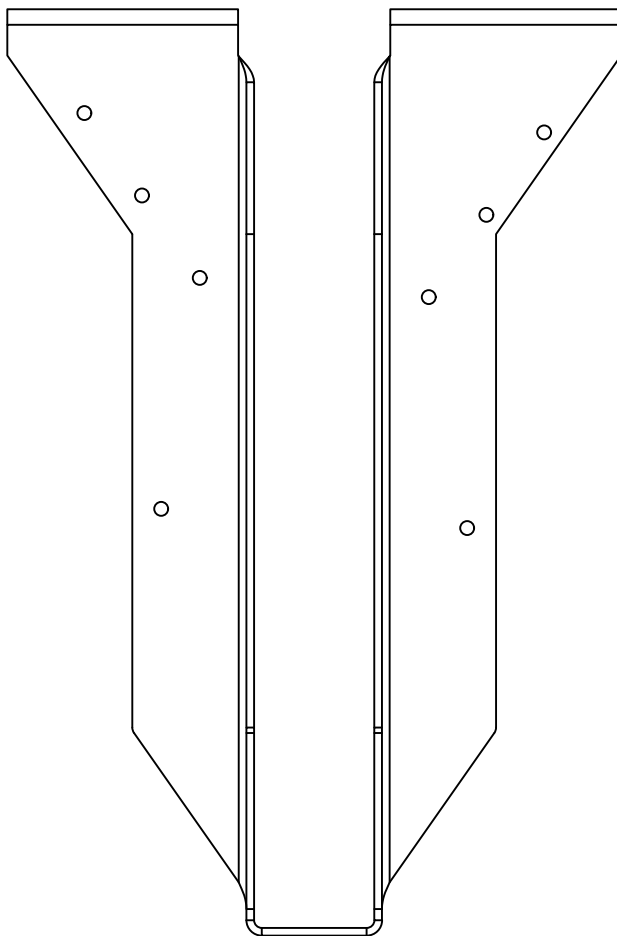
BPHA15118 - FRONT VIEW
