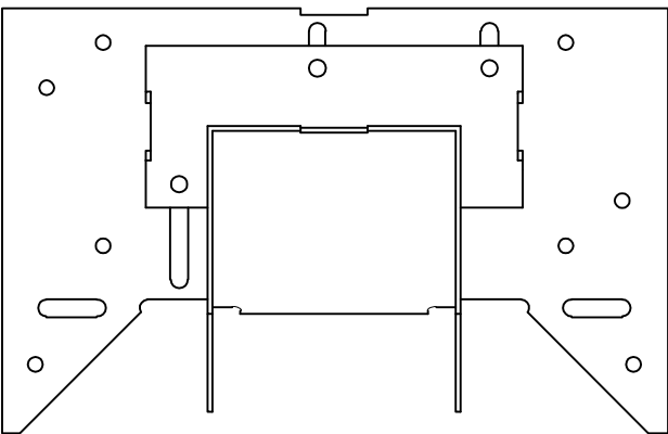
TMPH25 - FRONT VIEW
