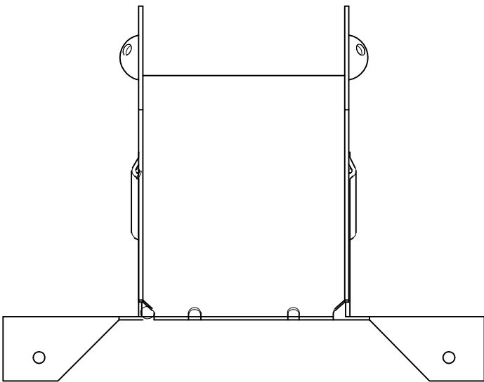
TMP25 - FRONT VIEW
