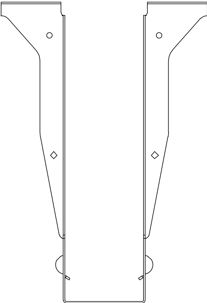
TFL2595 - FRONT VIEW
