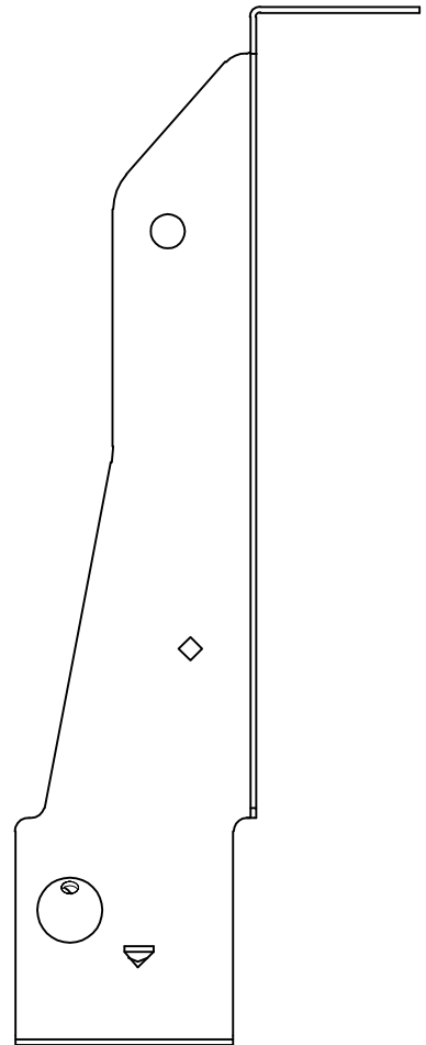
TFL25938 - SIDE VIEW
