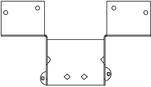
TFL2516 - TOP VIEW
