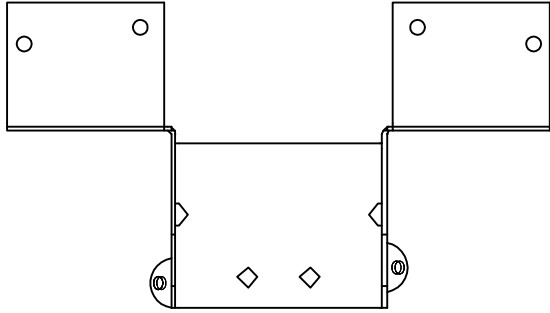
TFL2514 - TOP VIEW
