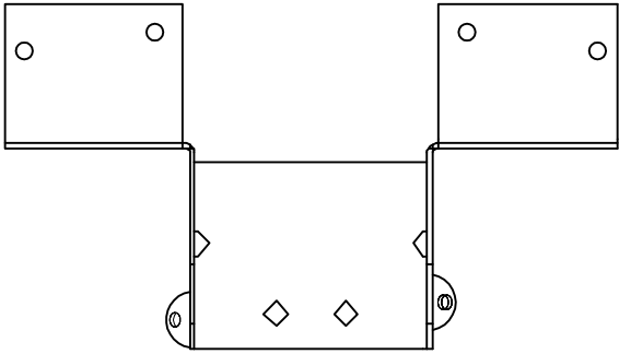
TFL2513 - TOP VIEW
