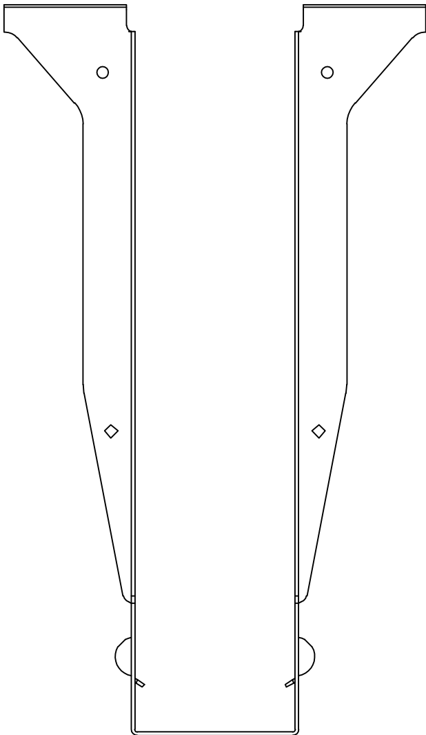
TFL25112 - FRONT VIEW
