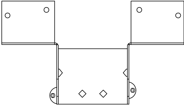
TFL25112 - TOP VIEW
