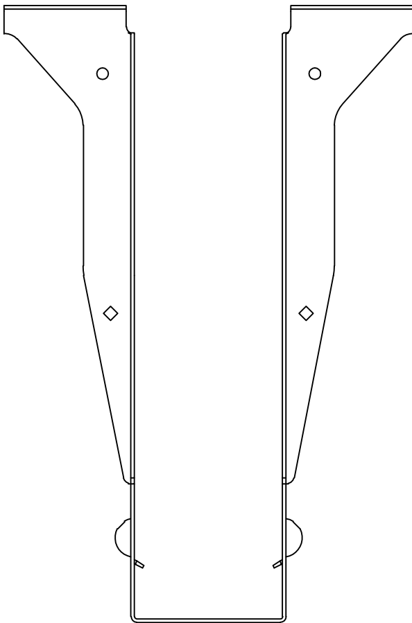
TFL23950 - FRONT VIEW
