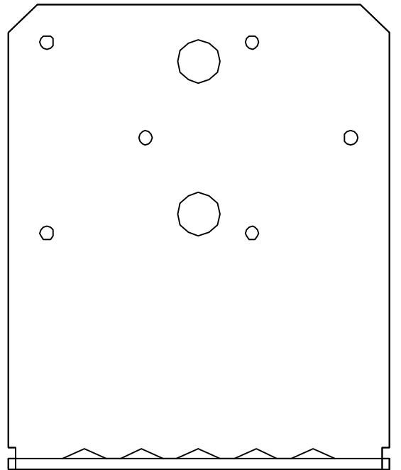
PAU46 - SIDE VIEW
