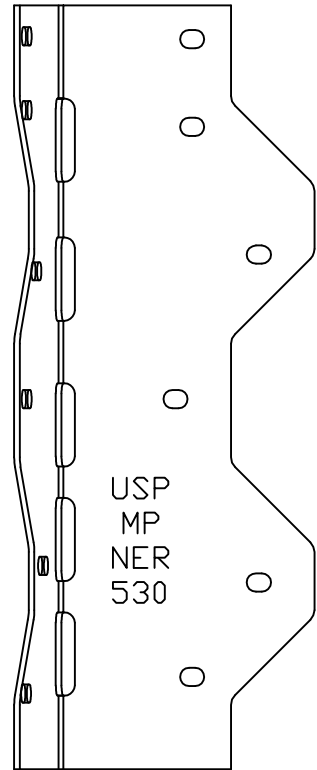
MP9 - FRONT VIEW
