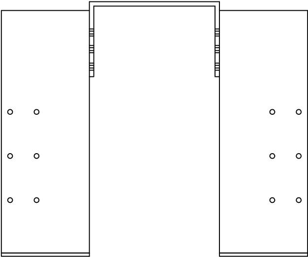
KGLS5-7 - SIDE VIEW
