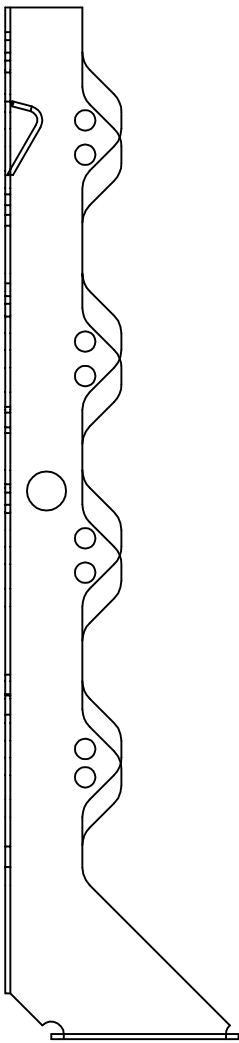
JL210 - SIDE VIEW
