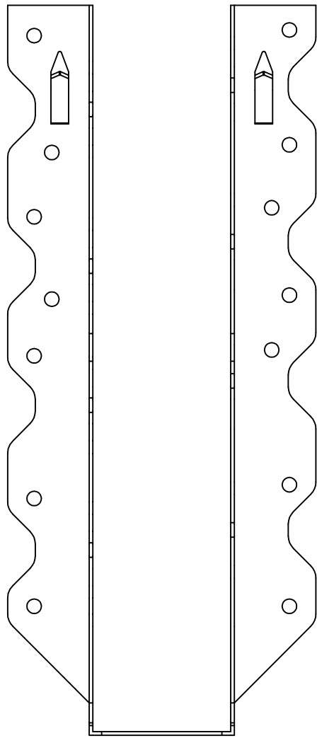
JL210 - FRONT VIEW
