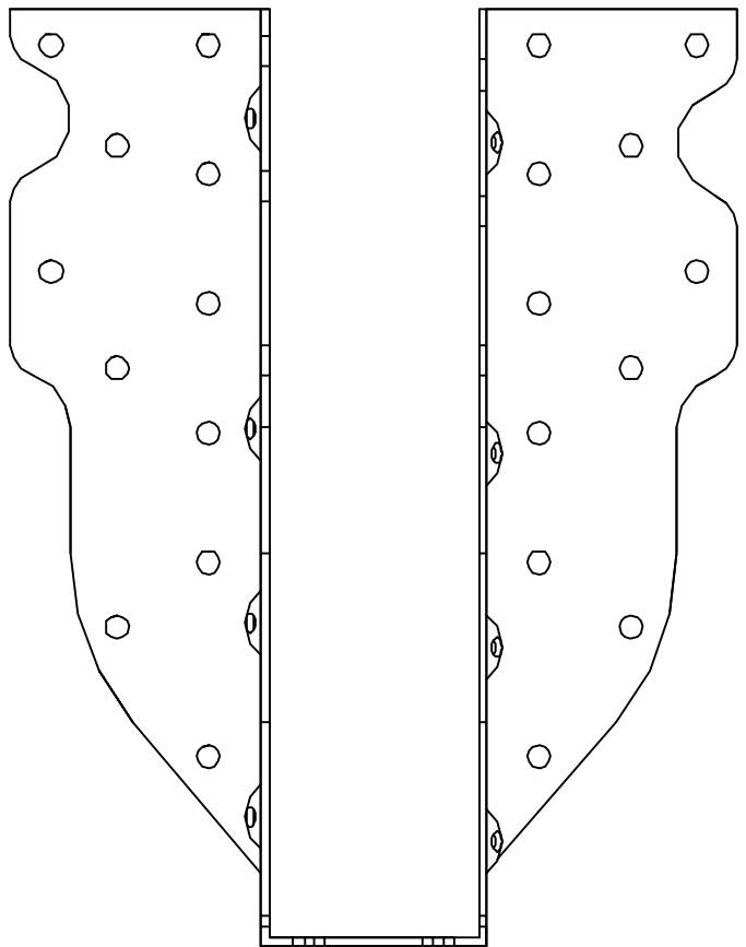
HUS28 - FRONT VIEW
