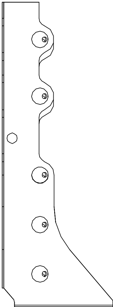
HUS210 - LEFT SIDE VIEW
