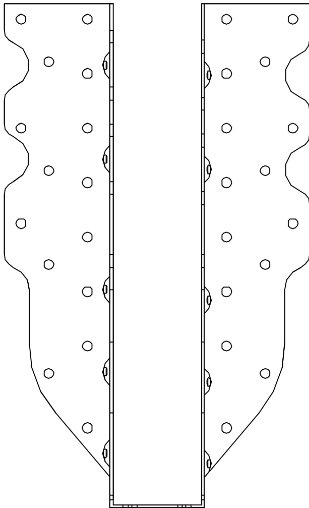
HUS210 - FRONT VIEW
