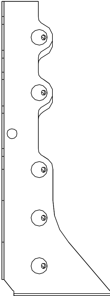
HUS179 - LEFT SIDE VIEW
