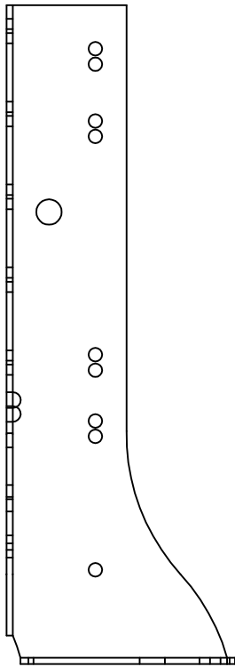
HD5210 - SIDE VIEW
