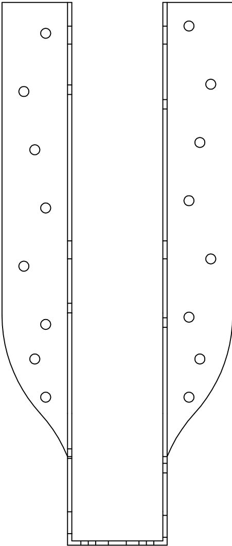
HD212 - FRONT VIEW
