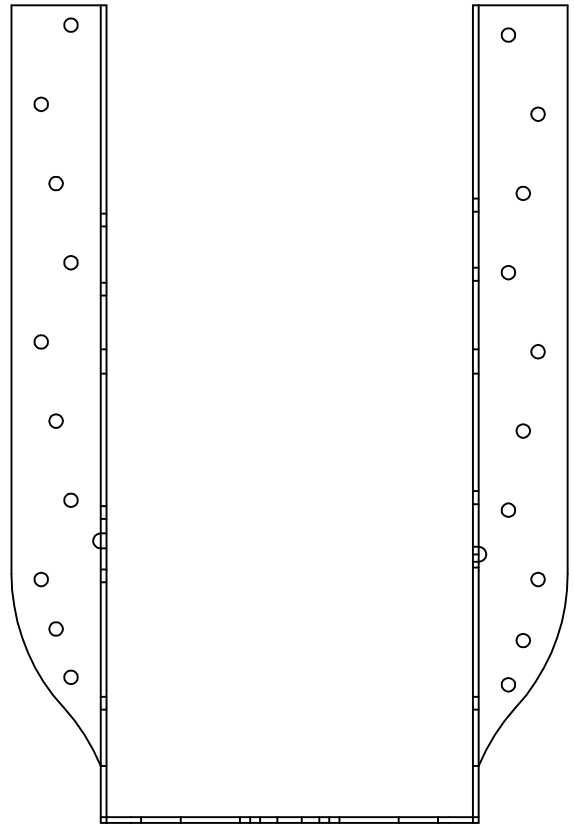
HD212-3 - FRONT VIEW
