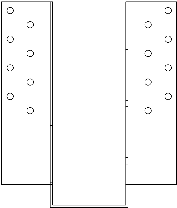
GHF31900 - FRONT VIEW
