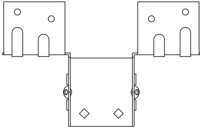
TH017950 - TOP VIEW
