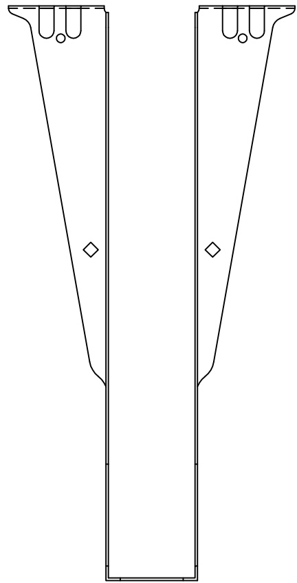
TH017118 - FRONT VIEW
