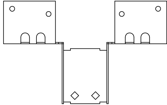
TH015950 - TOP VIEW
