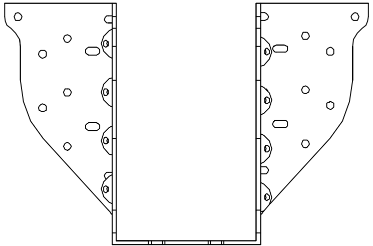
THDH26-2 - FRONT VIEW
