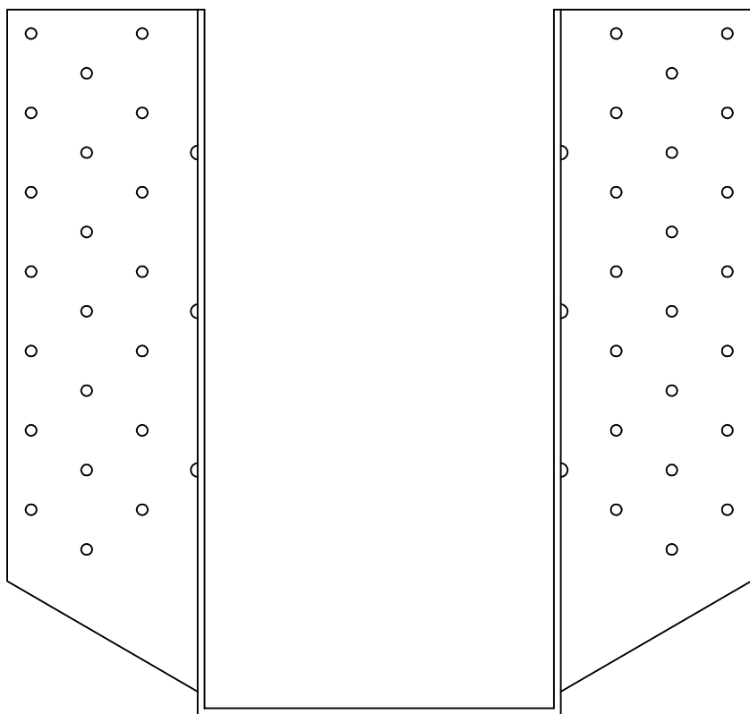
THD612 - FRONT VIEW
